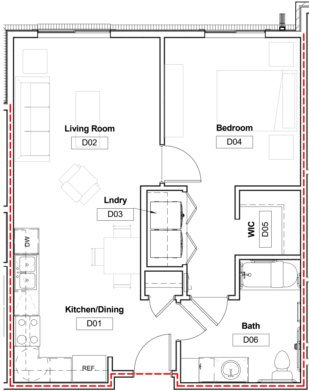
Unit Type 'D' : One Bedroom Handicap 704 SF
