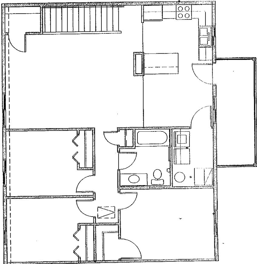
2 3 BDRM. UNIT ABOVE H/C SCALE: 3/16" = 1'-0" 1,194 SF
