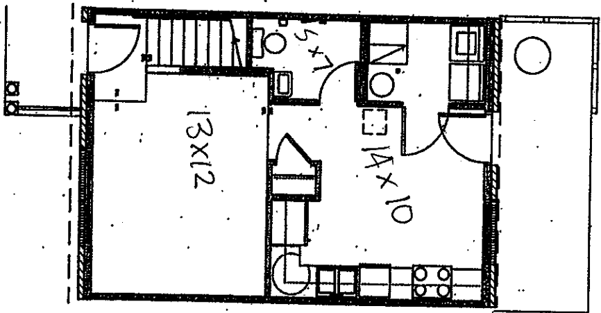
1 2 BDRM 1ST FLR SCALE: 3/16" = 1'-0" 486 SF
